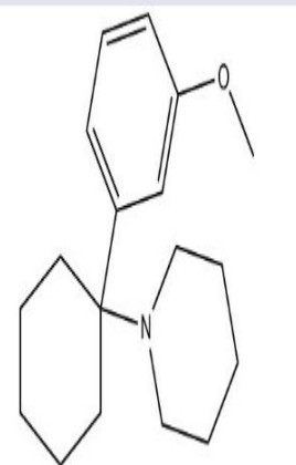
1-(1-(3-methoxyphenyl)cyclohexyl)piperidine
